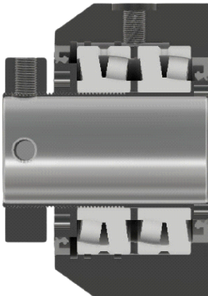
BILLET STEEL ROUND FLANGE BX-RF S-2000
